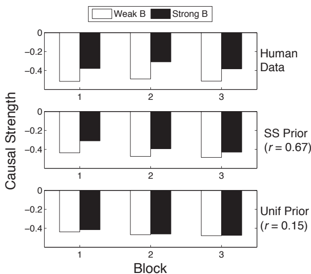
Figure 2: Human causal strength judgments for cause A and predictions from models using sparse-and-strong (SS) and uniform (Unif) priors across blocks.
