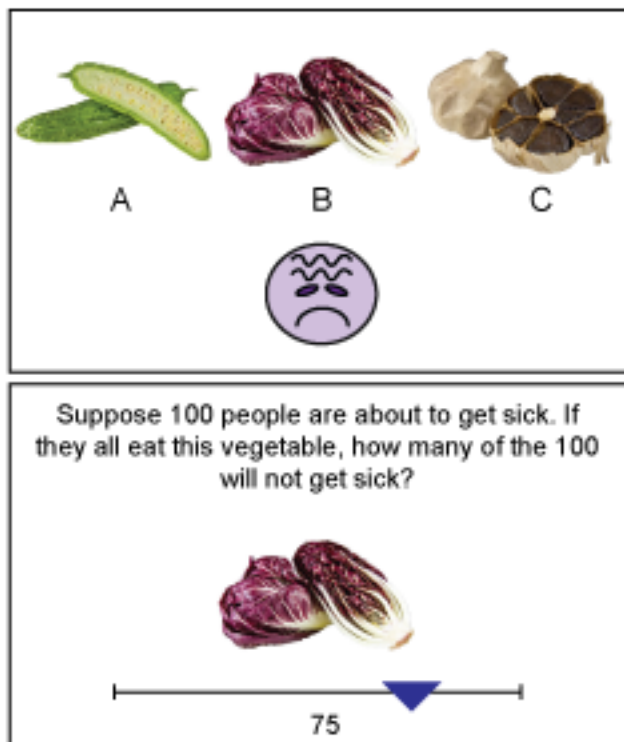
Figure 1: Example trial showing sick guest who ate A, B, and C vegetables (top). Example response trial for preventive cause (bottom).
