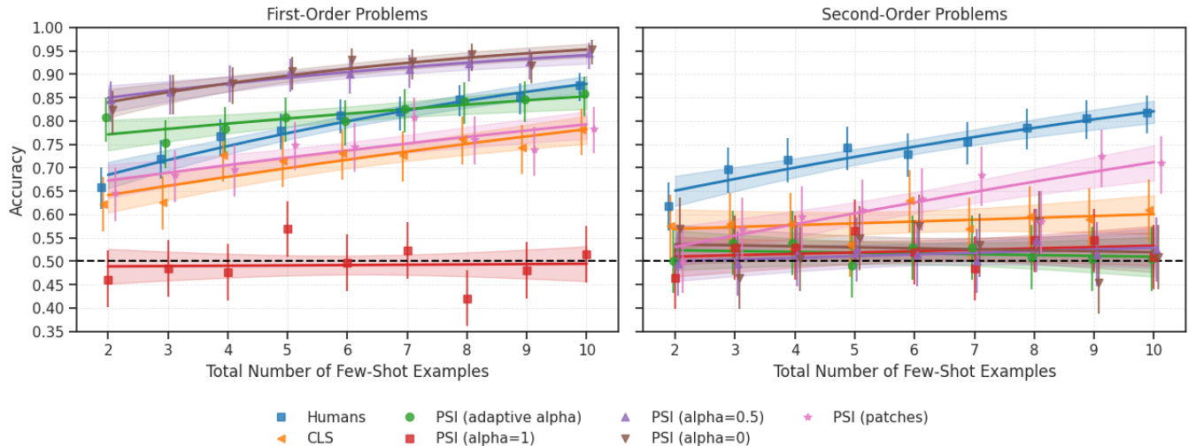
Figure 3: Accuracy by total number of few-shot examples, separately for first-order and second-order problems. Curves are logistic regressions. Error bars/bands are binomial 95% confidence intervals. Dashed lines indicate chance.
