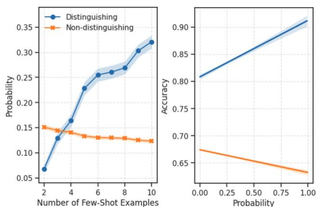
Figure 5. Edge weight (probability) by number of few-shot examples (left) and accuracy by edge weight (right), separately for class-distinguishing and non-distinguishing relations of a problem. Lines on the right reflect linear regressions. Error bands are 95% confidence intervals.
